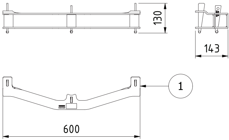
Figure 6. Stiffener
