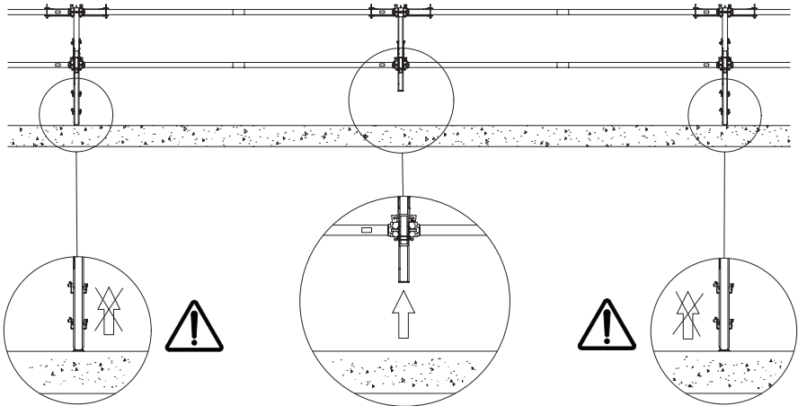
Figure 23. Only one Support Leg at a time is allowed to be lifted
