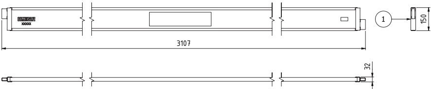
Figure 8. Toe Board
